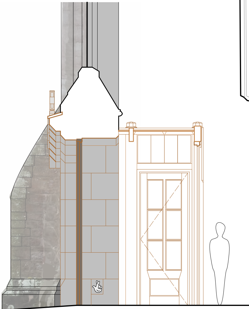
Section looking north
